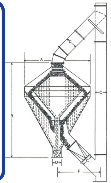
Square Cleaner Showing Round Cones
